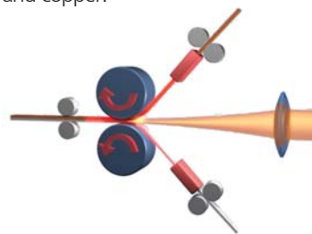
(below) Laser Induction Roll Plated Aluminum / Copper Joint
